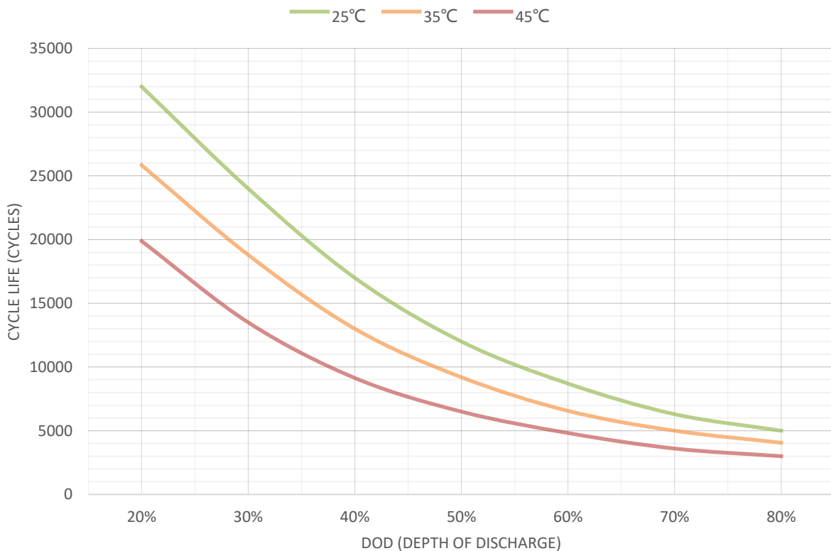
Cycle Life vs. DOD at Different Temperature
